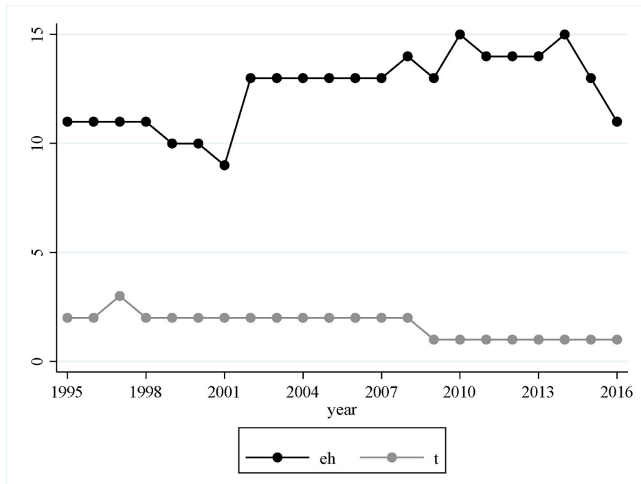
Fig. 3. CO 2 emissions by electricity and heat generation and transport sectors in Cuba. Notes: the Stata command twoway scatter was used to obtain this graph; the black dots represent CO 2 emissions from the electricity and heat generation sector (eh) while the grey dots represent CO 2 emissions from the transport sector (t), both from Cuba.
